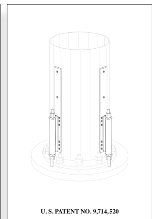
Direct Anchorage™ Termination
